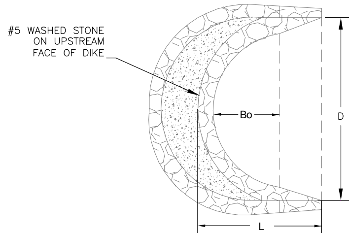
TYPICAL ROCK DIKE DIMENSIONS
